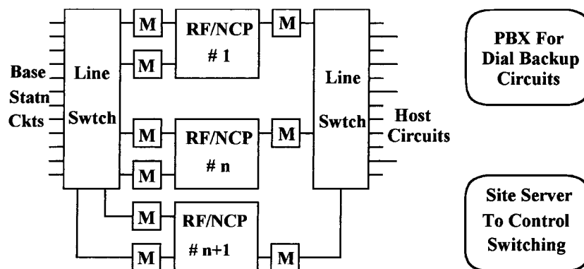
Figure 18-7 ARDIS licensed space arrangements (LSAs).
