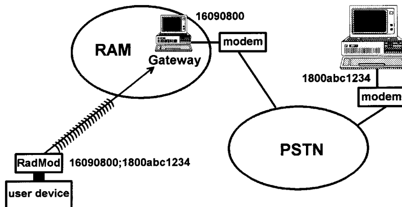
Figure 17-6 Wireless to PSTN to LAN.
