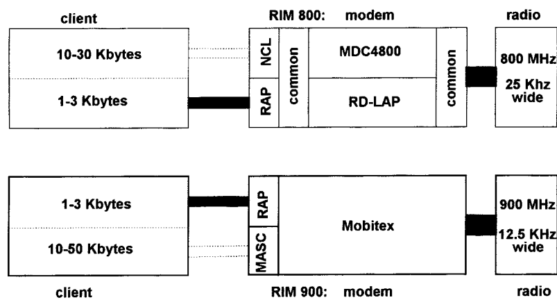
Figure 17-1 RAP interface in RIM X00 radio modems.
