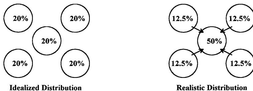
Figure 14-11 Busy-cell factor: 5 base ARDIS.
