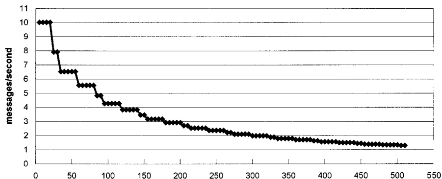
Figure 14-5 RD-LAP inbound message rate: offered traffic G = 80%.
