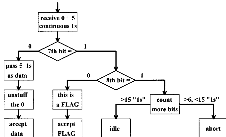
Figure 13-5 Bit stuffing.
