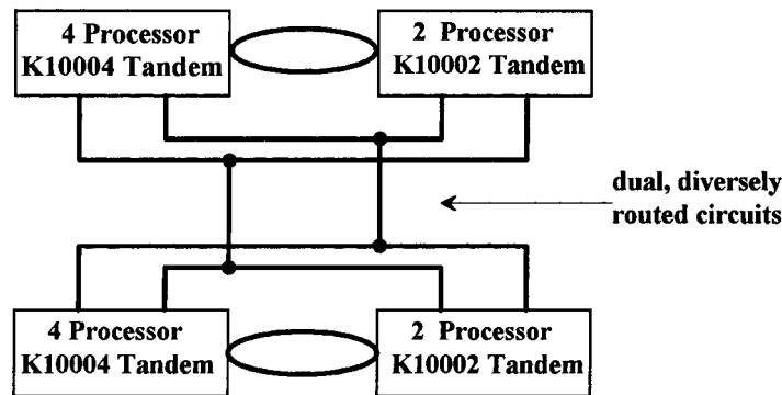
Figure 18-8 ARDIS switch linkage.
