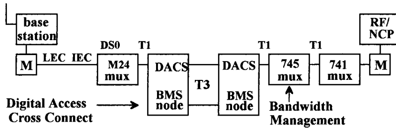
Figure 18-6 ARDIS base station to RF/NCP wireline configuration.
